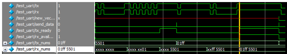
Figure 5.4: UART testbench waveform
